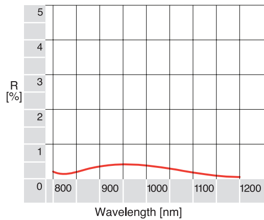
IR BROADBAND ANTI-REFLECTION COATING A66 (800-1200nm) ———
