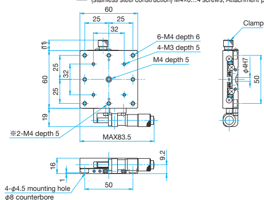
TSDH-602C Hexagonal socket head cap screw (stainless steel construction) M4x6...4 screws, Attachment pin for M4
