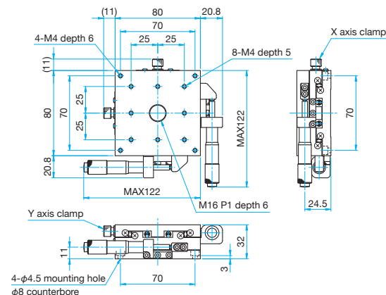
TSD-802SR Hexagonal socket head cap screw M4×8...4 screws
