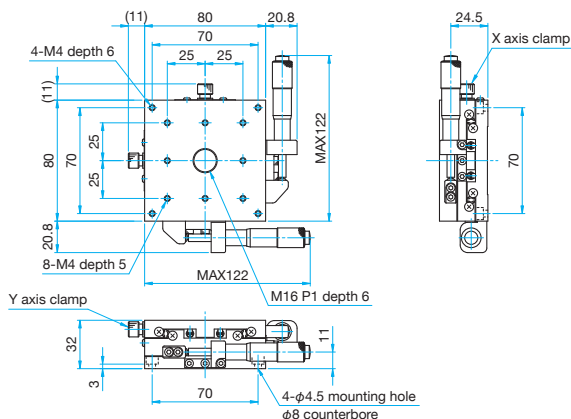
TSD-802S Hexagonal socket head cap screw M4×8...4 screws
