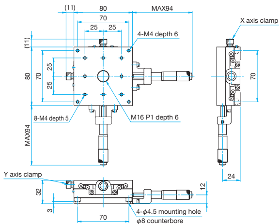
TSD-802S Hexagonal socket head cap screw M4×8...4 screws
