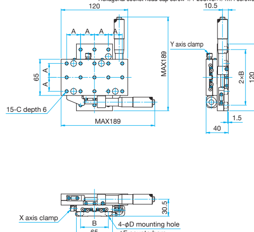
TSD-65122S-M6/65122SUU Hexagonal socket head cap screw M6×6...4 screws (M6) Hexagonal socket head cap screw 1/4-20UNC×1/4...4 screws (UU)
