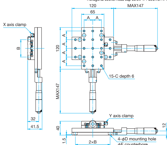
TSD-65122C-M6/65122CUU Hexagonal socket head cap screw M6×6...4 screws (M6) Hexagonal socket head cap screw 1/4-20UNC×1/4...4 screws (UU)
