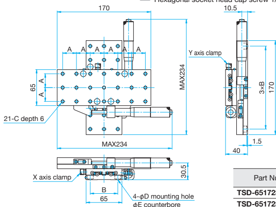
TSD-65172S-M6/65172SUU Hexagonal socket head cap screw M6×6...4 screws (M6) Hexagonal socket head cap screw 1/4-20UNC×1/4...4 screws (UU)
