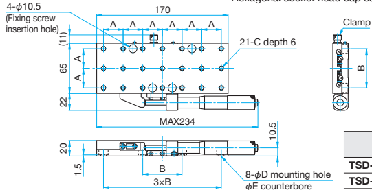
TSD-65122C-M6/65122CUU Hexagonal socket head cap screw M6×6...4 screws (M6) Hexagonal socket head cap screw 1/4-20UNC×1/4...4 screws (UU)
