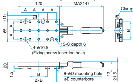
TSD-65121C-M6/65121CUU Hexagonal socket head cap screw M6×6...4 screws (M6) Hexagonal socket head cap screw 1/4-20UNC×1/4...4 screws (UU)
