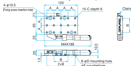
TSD-65121S-M6/65121SUU Hexagonal socket head cap screw M6×6...4 screws (M6) Hexagonal socket head cap screw 1/4-20UNC×1/4...4 screws (UU)
