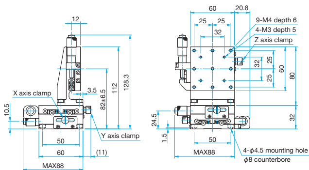
TSD-605SL Hexagonal socket head cap screw M4×6...4 screws
