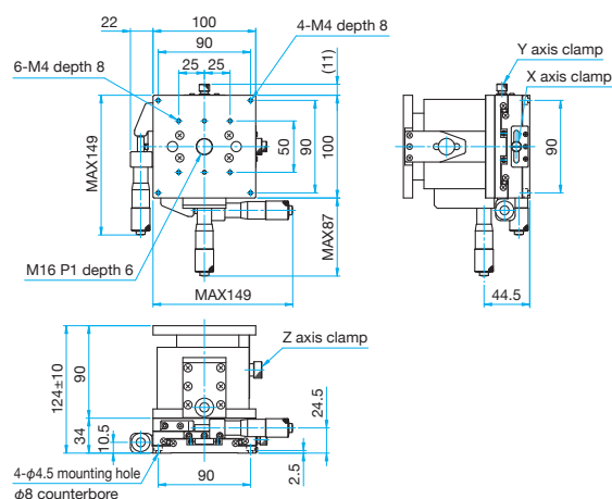
TSD-1005S Hexagonal socket head cap screw M4×8...4 screws
