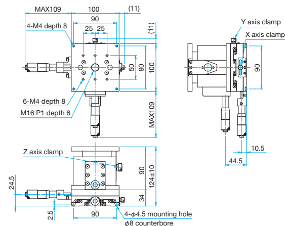
TSD-1005S Hexagonal socket head cap screw M4×8...4 screws
