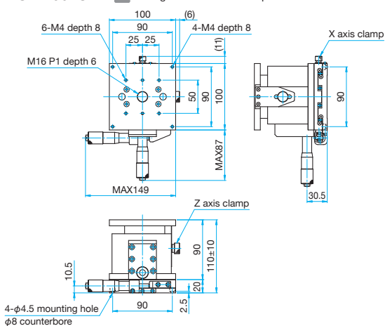
TSD-1004SR Hexagonal socket head cap screw M4×8...4 screws
