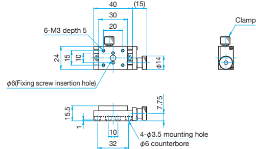
TAS-24301R Pan head screw M3×5...4 screws
