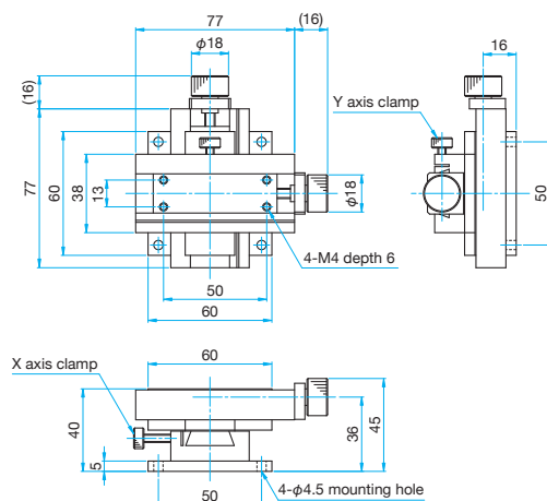
TAS-20602R Hexagonal socket head cap screw M4×10...4 screws
