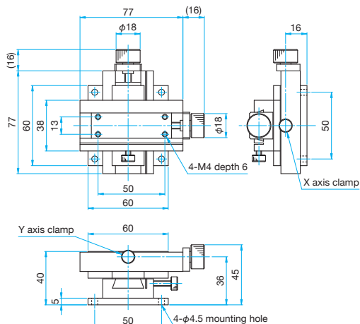
TAS-20602 Hexagonal socket head cap screw M4×10...4 screws
