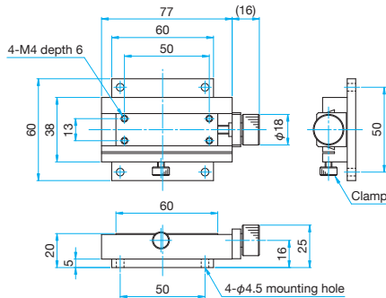
TAS-20601 Hexagonal socket head cap screw M4×10...4 screws
