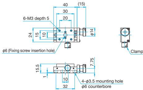
TAS-24301 Pan head screw M3×5...4 screws
