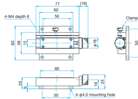
TAS-20601R Hexagonal socket head cap screw M4×10...4 screws
