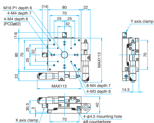
TAM-802SR Hexagonal socket head cap screw M4×8...4 screws
