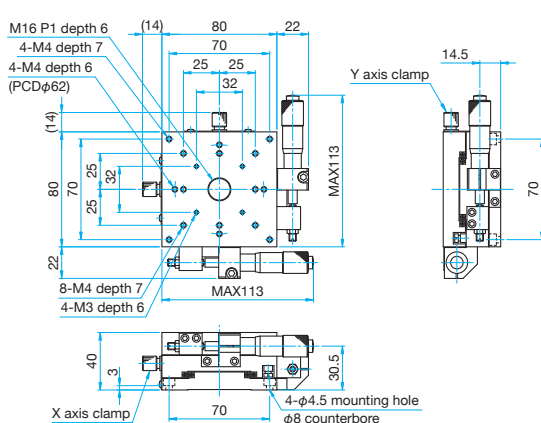
TAM-802S Hexagonal socket head cap screw M4×8...4 screws
