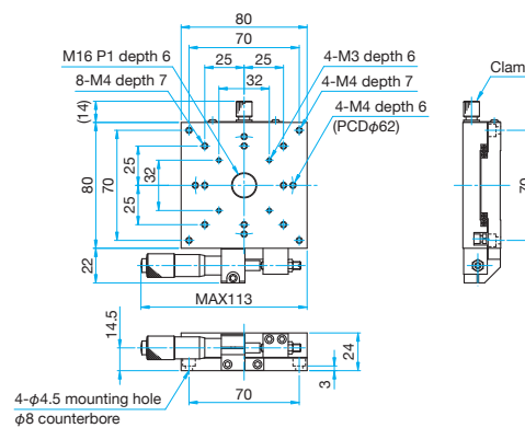
TAM-801SR Hexagonal socket head cap screw M4×8...4 screws
