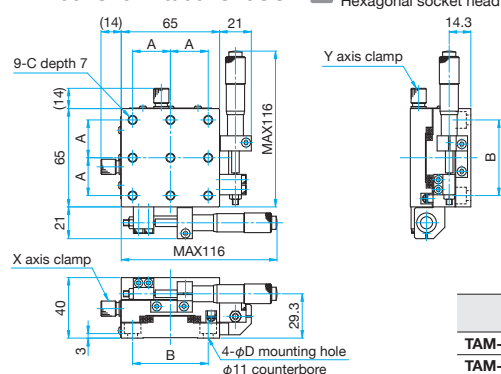
TAM-652S25-M6/652S25UU
