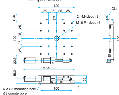
TAM-1201SR Hexagonal socket head cap screw M4×8...4 screws, Spring washers
