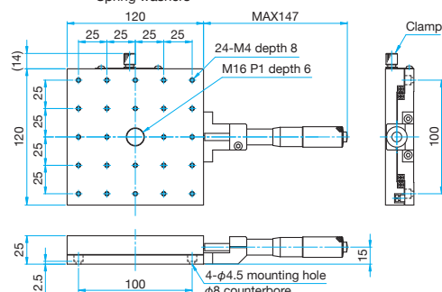
TAM-1201C Hexagonal socket head cap screw M4×8...4 screws, Spring washers
