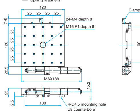
TAM-1201S Hexagonal socket head cap screw M4×8...4 screws, Spring washers
