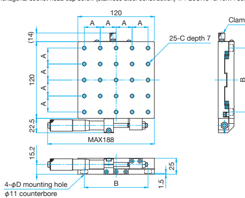
TAM-1201SR-M6/1201SRUU
