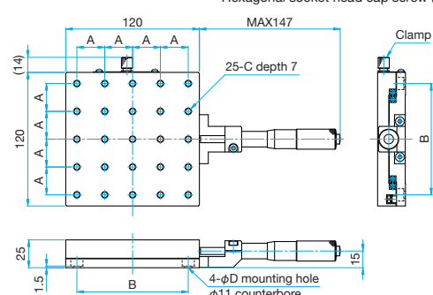
TAM-1201C-M6/1201CUU Hexagonal socket head cap screw M6×8...4 screws (M6) Hexagonal socket head cap screw (stainless steel construction) 1/4-20UNC×5/16...4 screws (UU)
