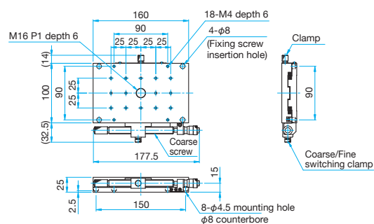
TAM-10161SR Hexagonal socket head cap screw M4×8...4 screws, Spring washers
