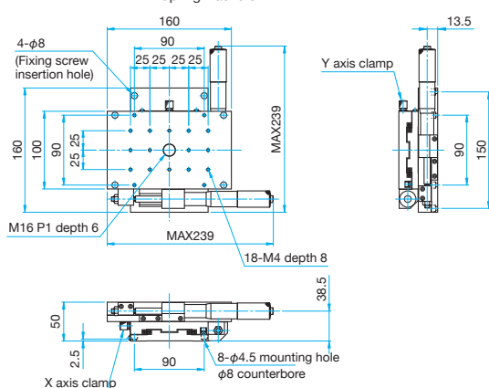
TAM-10162S Hexagonal socket head cap screw M4×8...4 screws, Spring washers
