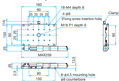
TAM-10162C Hexagonal socket head cap screw M4×8...4 screws, Spring washers
