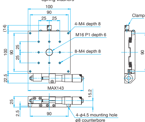
TAM-1002C Hexagonal socket head cap screw M4×8...4 screws, Spring washers
