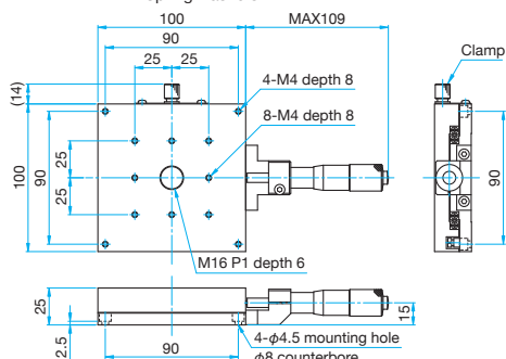
TAM-1001S Hexagonal socket head cap screw M4×8...4 screws, Spring washers
