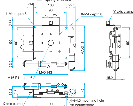
TAM-1002SR Hexagonal socket head cap screw M4×8...4 screws, Spring washers
