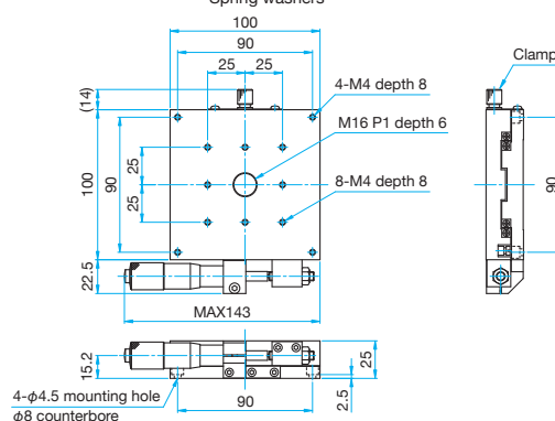
TAM-1001SR Hexagonal socket head cap screw M4×8...4 screws, Spring washers
