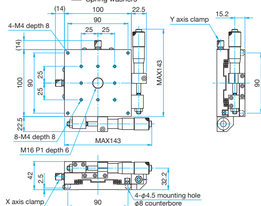
TAM-1002S Hexagonal socket head cap screw M4×8...4 screws, Spring washers
