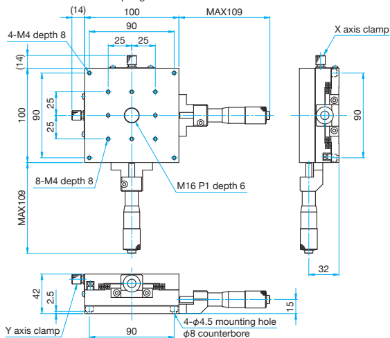
TAM-1002S Hexagonal socket head cap screw M4×8...4 screws, Spring washers
