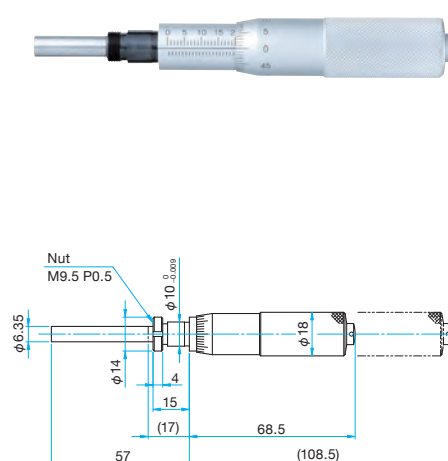
SHN2-40
