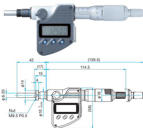
MHN2-25M
