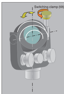
Tilt (pitch) coarse movement control
